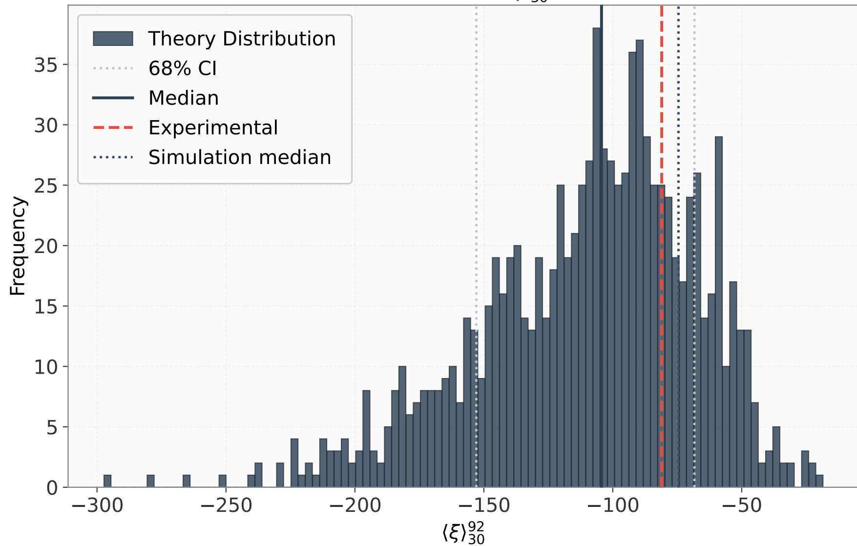
Distribution: \langle \xi \rangle_{30}^{92}
