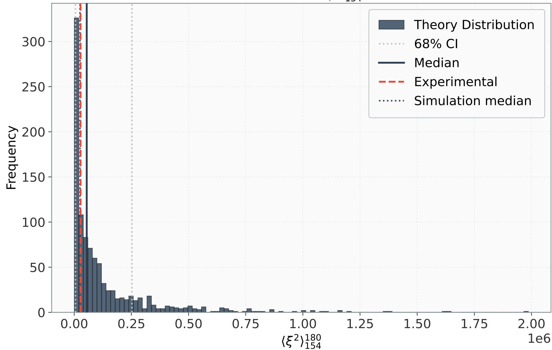
Distribution: \langle \xi^2 \rangle_{154}^{180}
