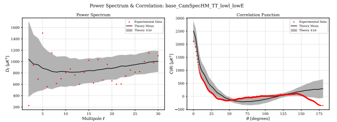
Figure 1: Power spectrum and correlation function
