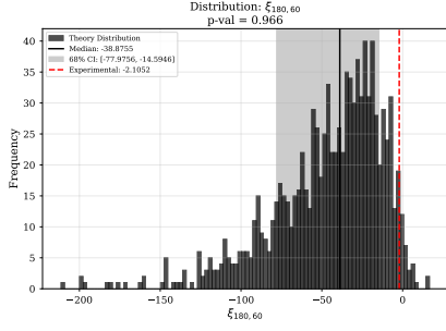
(a) \langle \xi \rangle_{60}^{180}
