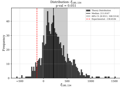
(b) \langle \xi \rangle_{154}^{180}
