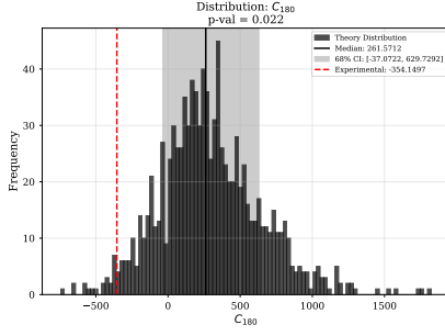
Figure 4: Best-fit Monte Carlo distribution of the antipodal correlation C_{180} for model base_CamSpecHM_TT_low1_lowE .
