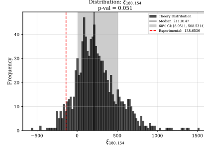
(b) \langle \xi \rangle_{154}^{180}
