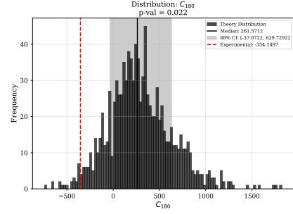
Figure 7: MCMC posterior distribution of C_{180} for model base_CamSpecHM_TT_lowl_lowE .
