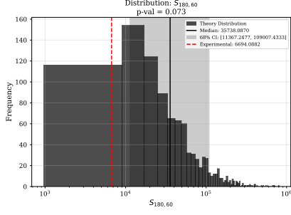
(a) S_{60}^{180} (classic S_{1/2} )
