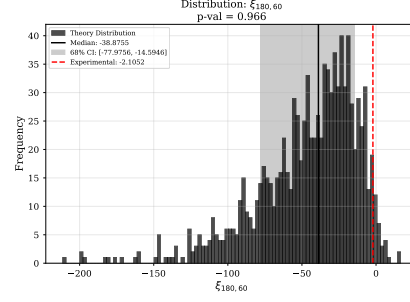
(a) \langle \xi \rangle_{60}^{180}
