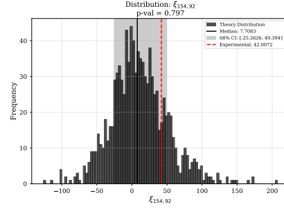
(c) \langle \xi \rangle_{92}^{154}
