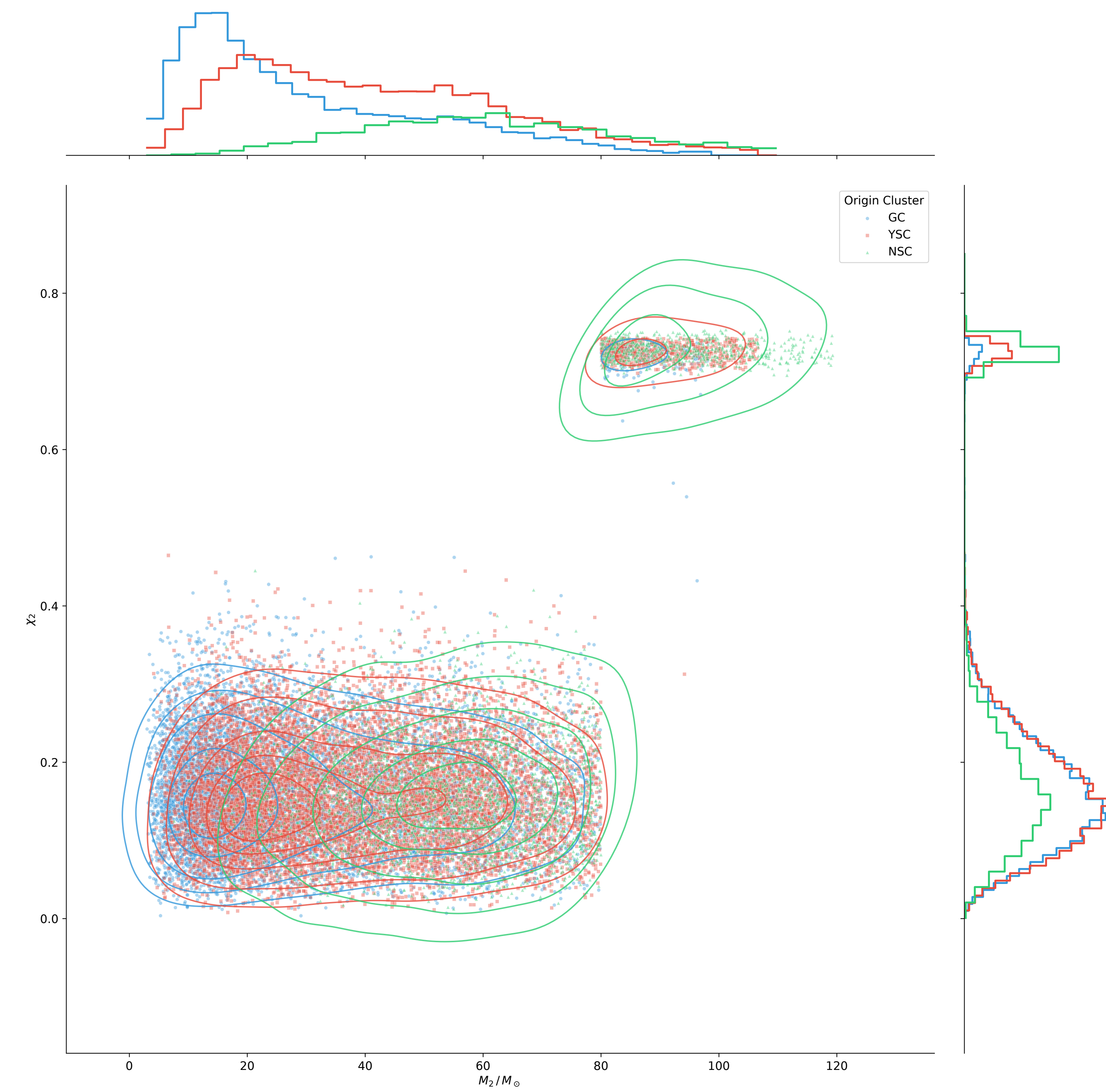
N_{\text{gen}} > 2 \mid 0.0002 \leq Z < 0.0012
