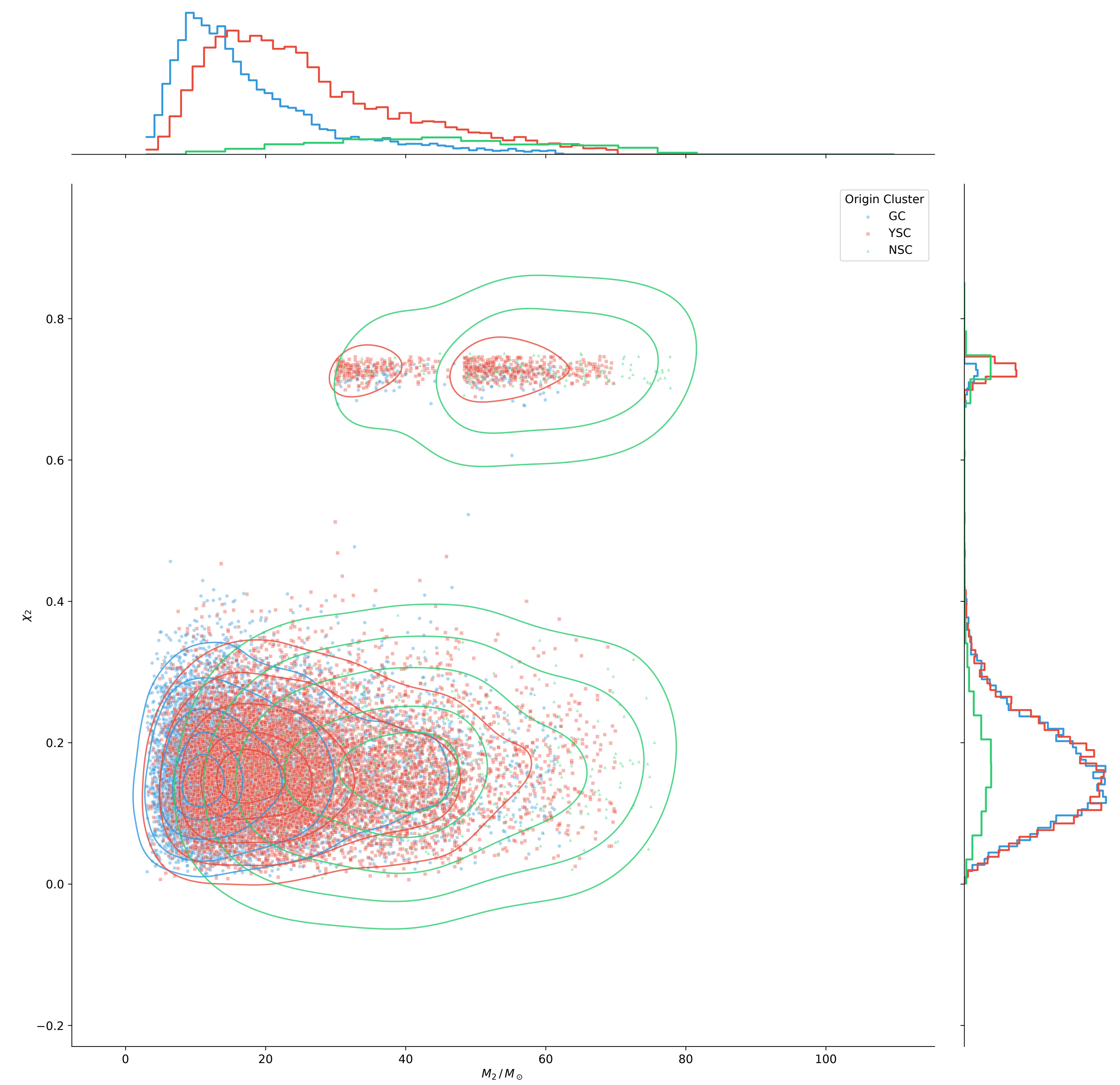
N_{\text{gen}} > 2 \mid 0.008 \leq Z < 0.3
