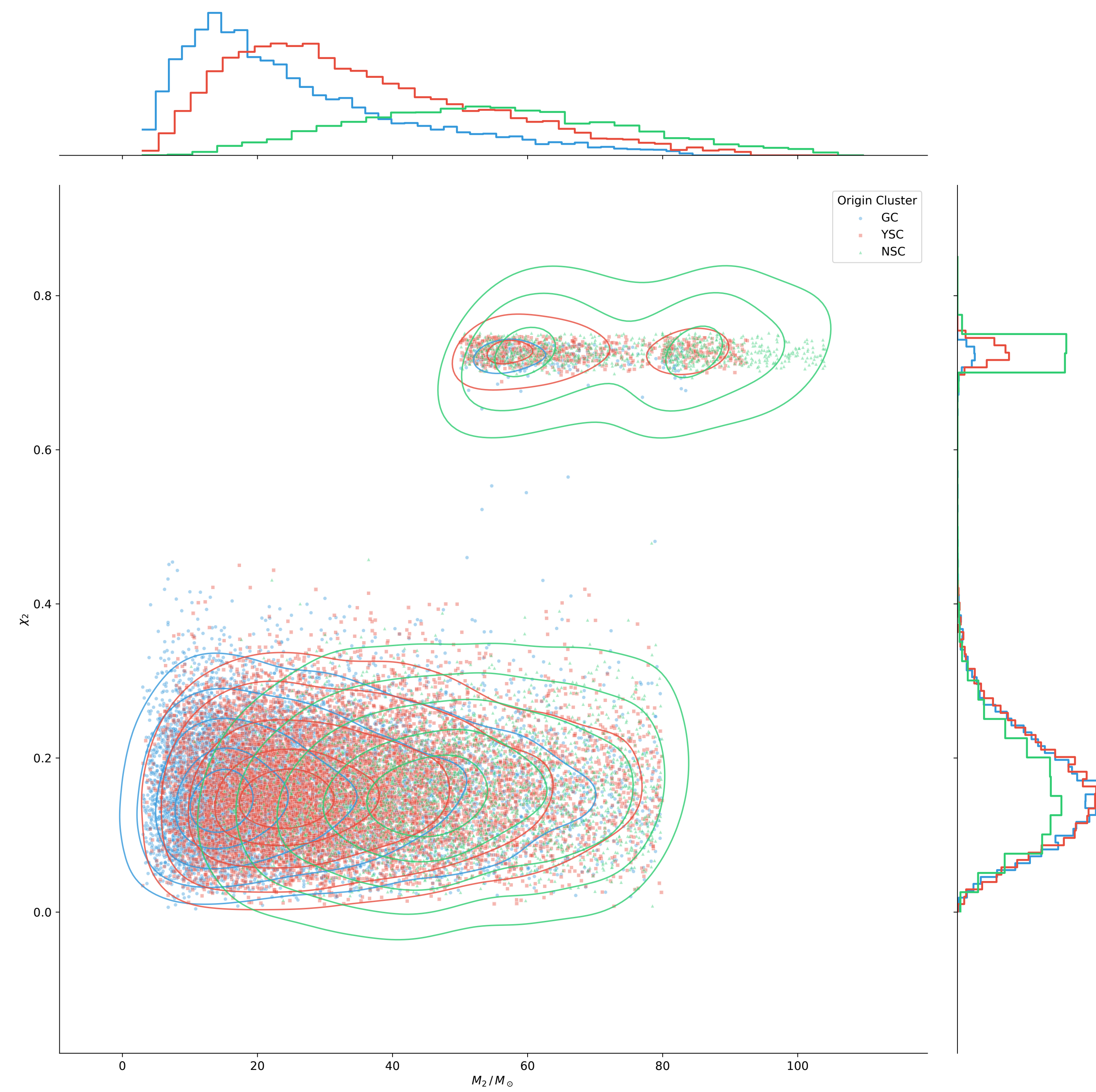
N_{\text{gen}} > 2 \mid 0.0012 \leq Z < 0.008
