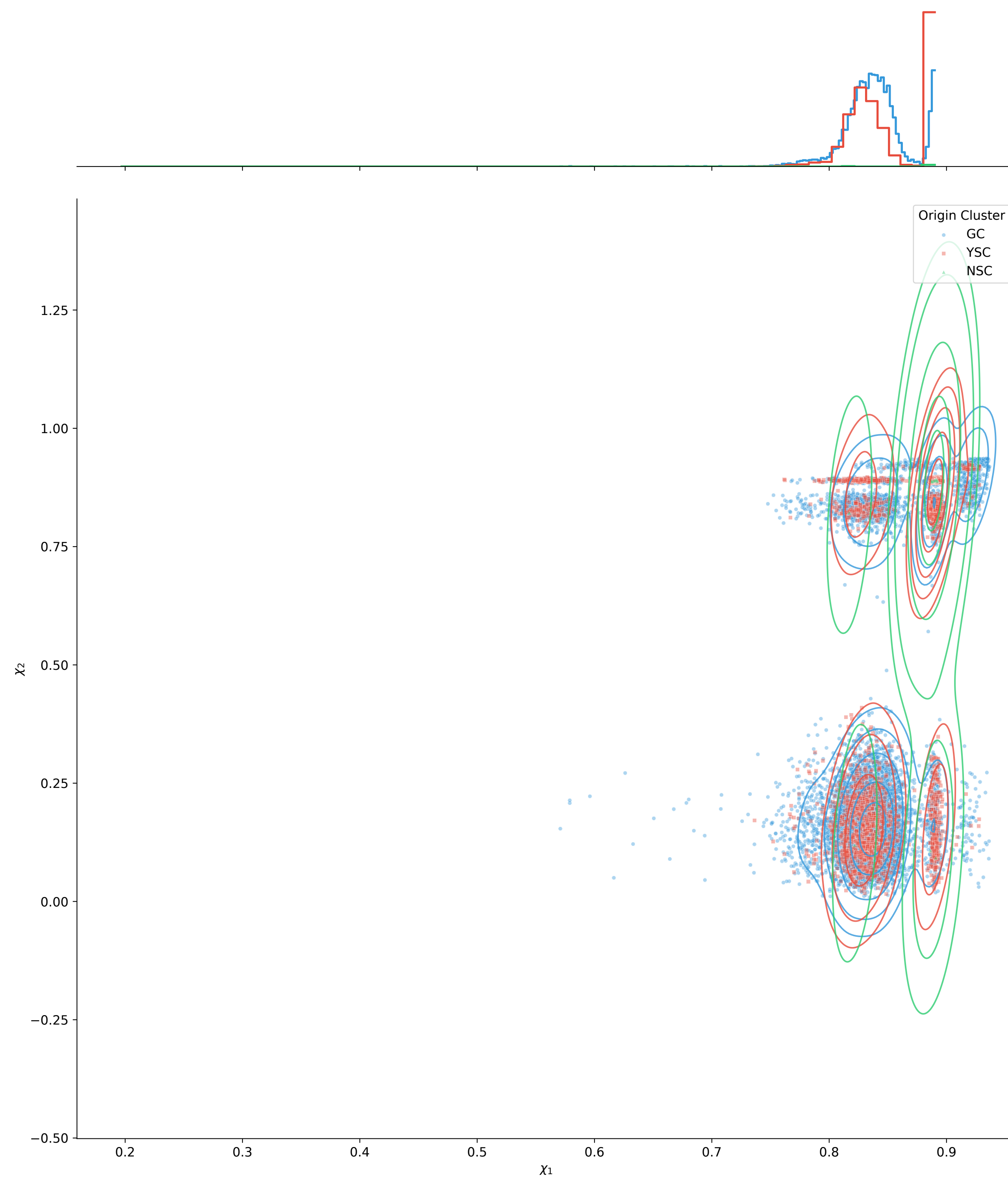
N_{\text{gen}} > 2 \mid 0.0012 \leq Z < 0.008
