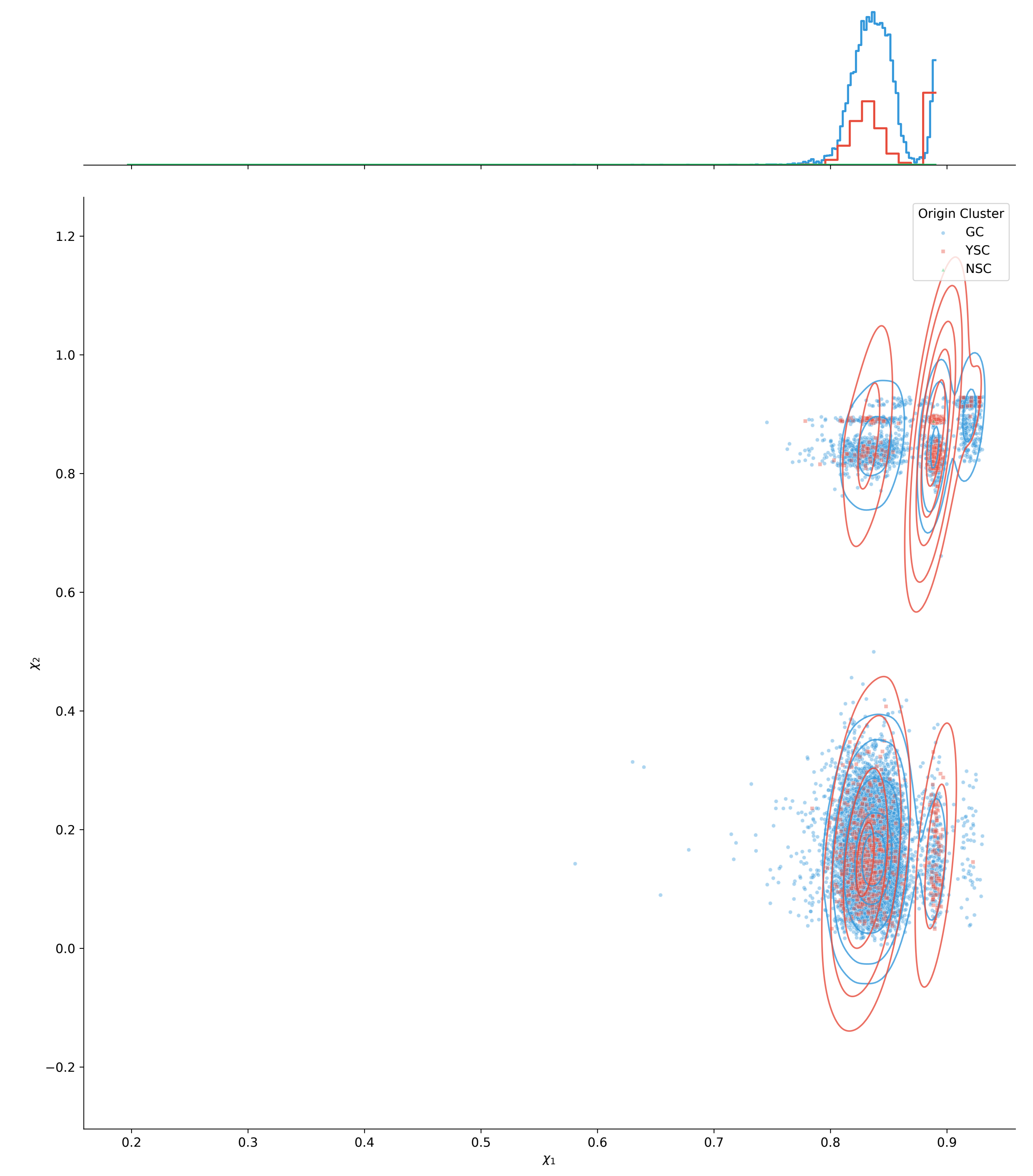
N_{\text{gen}} > 2 \mid 0.008 \leq Z < 0.3
