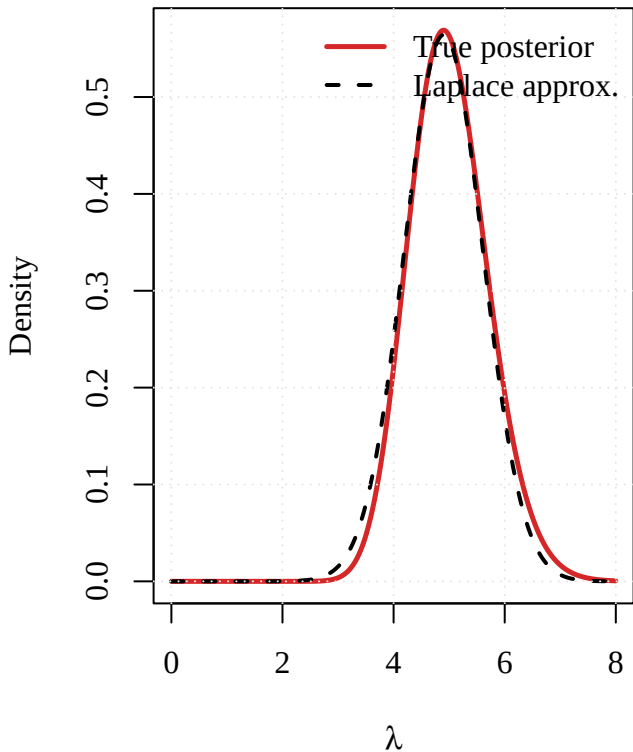
Well-peaked Gamma(50,10)
