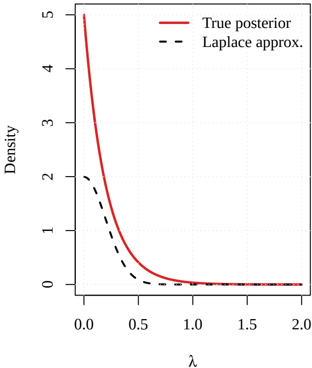
Broad Gamma(1,5) [zero counts]
