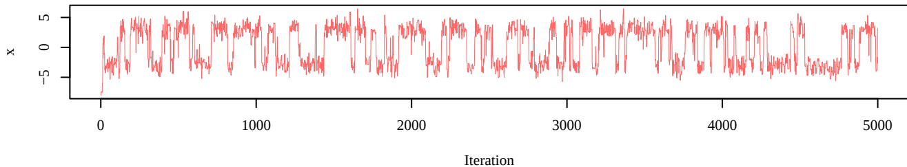
After burn-in
