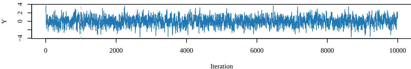
Posterior samples after burn-in
