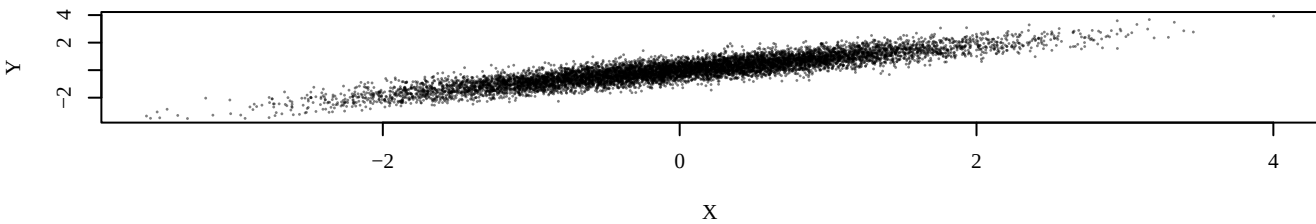
Posterior samples (rotated Gibbs)
