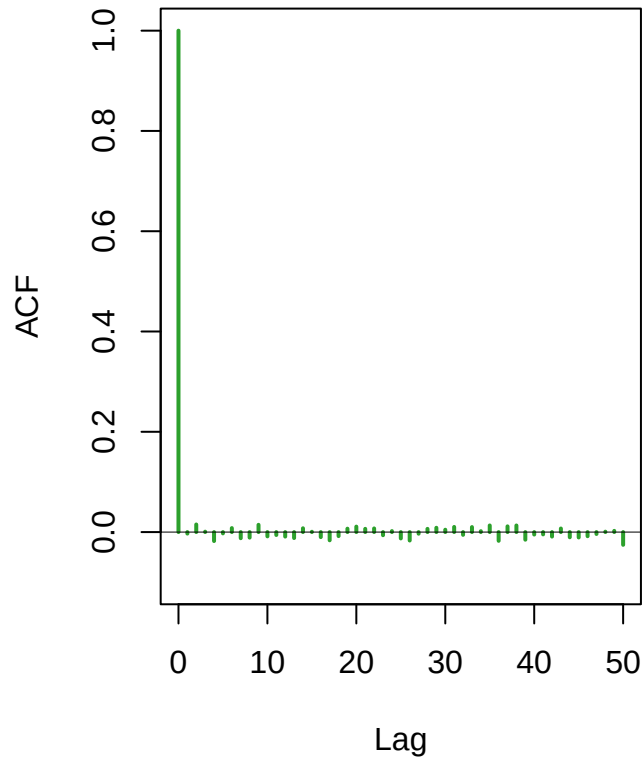
Rotated Gibbs ( \rho = 0.9 )
