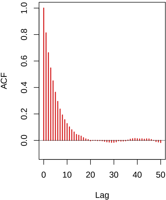
Standard Gibbs ( \rho = 0.9 )
