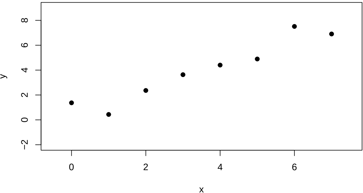
Linear Regression Data
