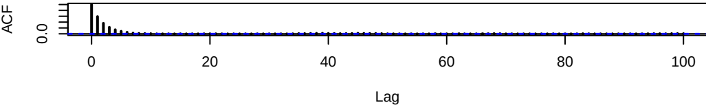
Autocorrelation: Independence Sampler
