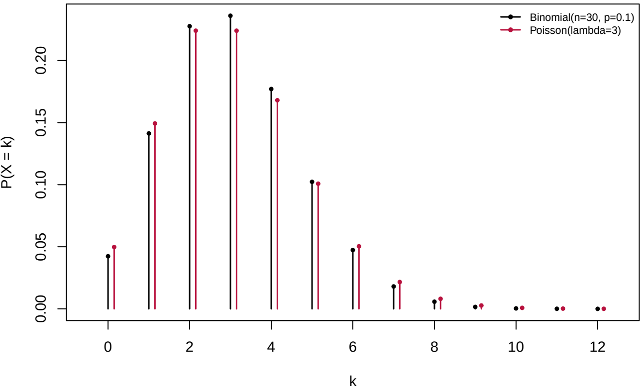
Poisson limit: Binomial( n=30 , p=0.1 ) vs Poisson( \lambda=3 )
