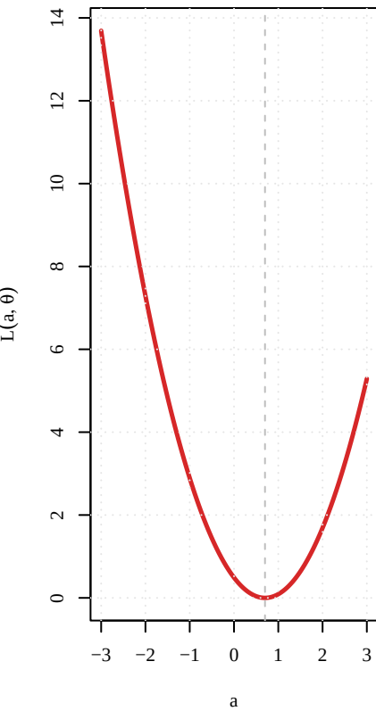
Squared Loss
