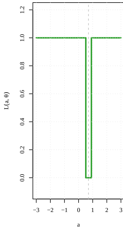
0-1 Loss
