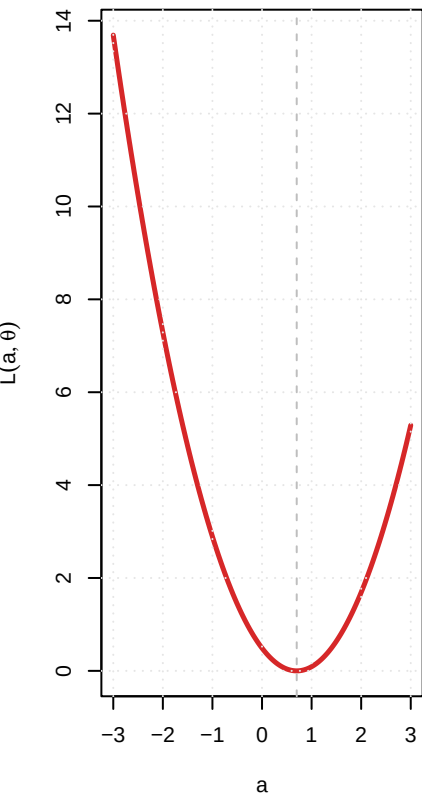
Squared Loss
