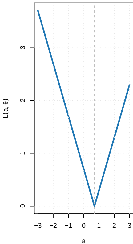
Absolute Loss
