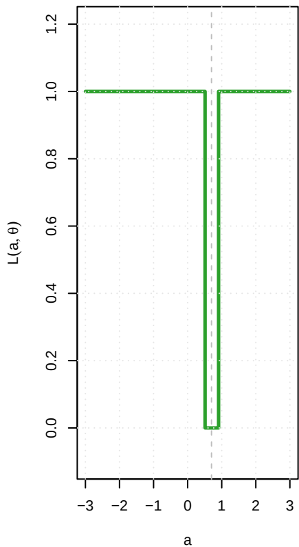
0-1 Loss
