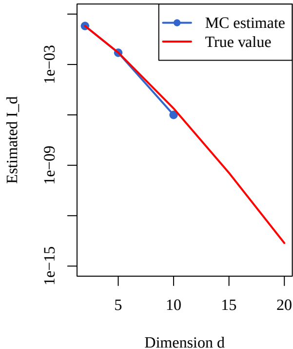
Hypersphere volume (log scale)
