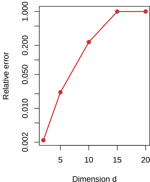
Relative error (log scale)
