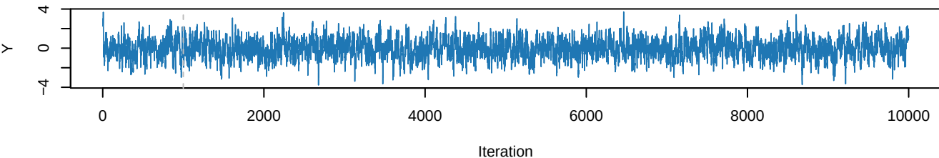
Posterior samples after burn-in
