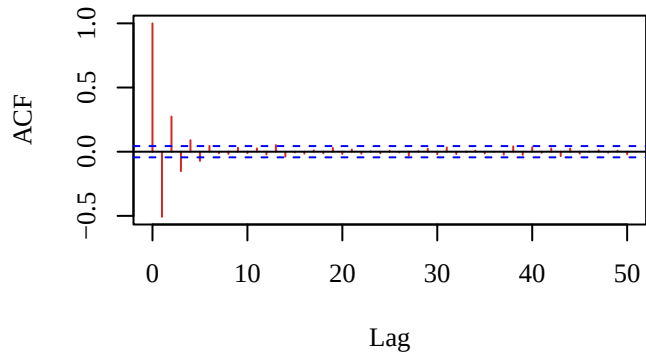
HMC Autocorr
