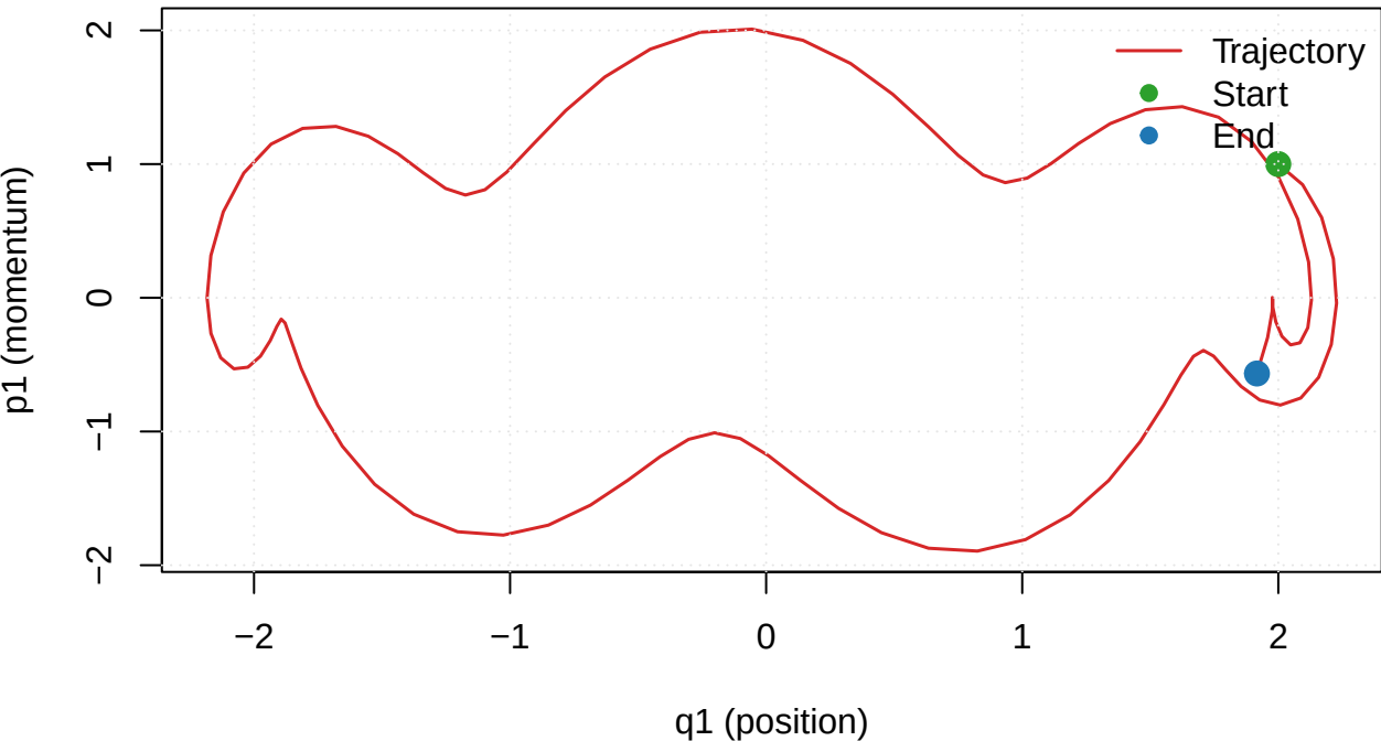
Leapfrog Trajectory in Phase Space ( q_1 , p_1 )
