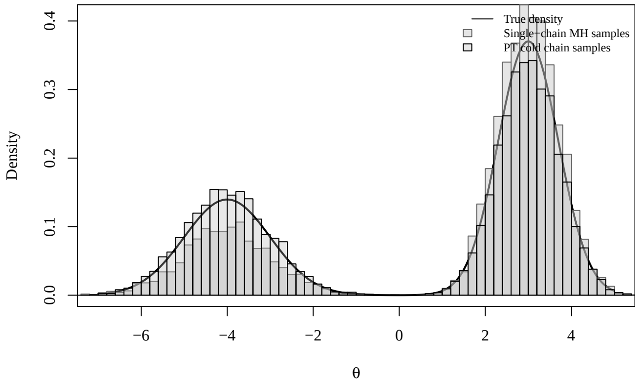
Posterior: true density vs. samples
