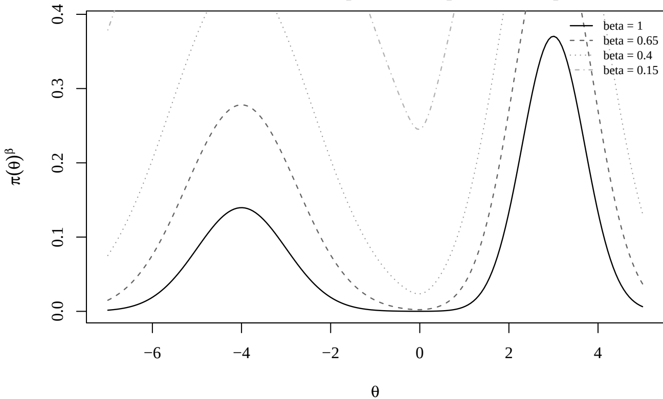
Effect of inverse temperature on posterior shape
