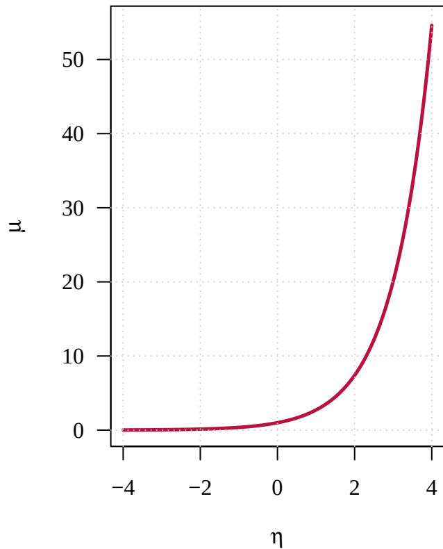
Log inverse link
