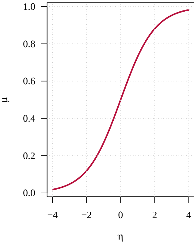
Logit inverse link
