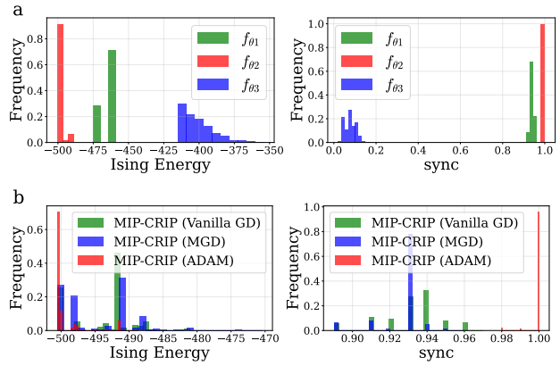
Figure 2. Comparison of attractor classes on a 100-spin Ising model with 1000 random initializations. (a) The quartic attractor f_{\theta_2} (red) significantly outperforms quadratic f_{\theta_1} (green) and mean-field based f_{\theta_3} (blue) attractors, yielding the lowest Ising energy while achieving synchronization score \text{sync} = 1 (29) almost every time. (b) Evaluation of first-order optimizers \mathcal{O} (used in Algorithm 1) using the quartic attractor f_{\theta_2} . ADAM (red) demonstrates superior convergence properties, achieving the best synchronization score ( \text{sync} = 1 ) always (along with the lowest Ising energy), each time and consistently lower energy states compared to Momentum Gradient Descent (MGD) and Vanilla GD. The results are obtained using NVIDIA L40S GPU with Intel Xeon 6520P CPU.
