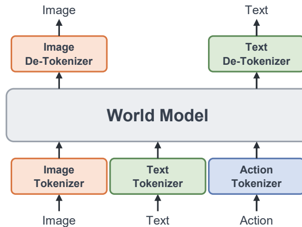
(b) World Model (e.g., iVideoGPT)
