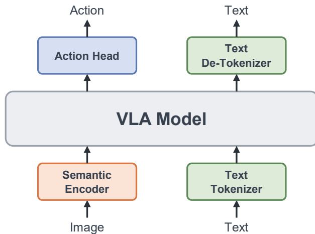
(a) VLA Model (e.g., OpenVLA)
