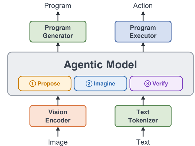
(c) Agentic Model (e.g., AGI (ours))
