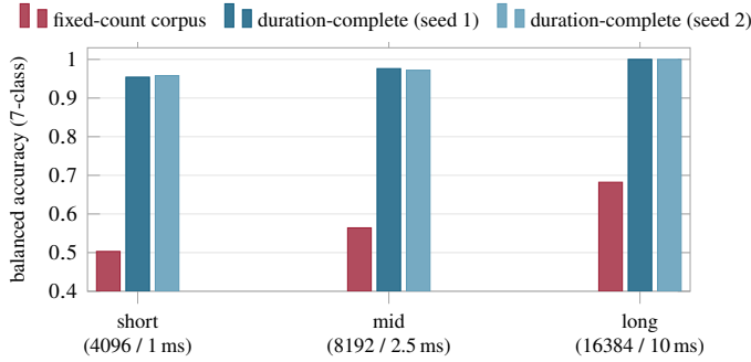
Figure 6: Controlled attribution. The identical 1.0M-parameter encoder, recipe, and budget on the fixed-count control corpus (window tiers in samples) vs. duration-complete data (dwells in milliseconds); tiers are matched by rank, not physical duration, which fixed-count data cannot hold constant. At 10 ms every class reaches recall 1.000 on both seeds.
