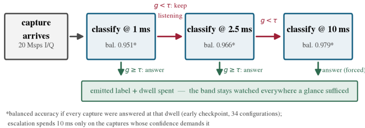
Figure 4: The dwell policy, traced (Algorithm 2). Each capture is classified at 1 ms; the confidence head either emits the answer or extends the dwell. Balanced accuracies are measured (early checkpoint); escalation spends 10 ms only where confidence demands it, so the monitor’s sweep budget survives.
