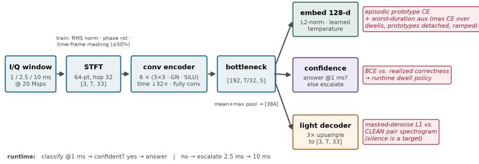
Figure 5: The DACS network. One shared spectro-temporal encoder; three heads. The prototype embedding [3] carries classification and preserves enrollment-based open-set operation; the confidence head [6, 8] drives the answer-early/escalate dwell policy; the light decoder reconstructs the clean reference’s spectrogram under time-frame masking [4, 5], making silence a learning target and regularizing against the shortcut overfit that duration-starved training exhibits (Sec. 6). The worst-case-over-dwell auxiliary trains the shortest dwell against its hardest cases.
