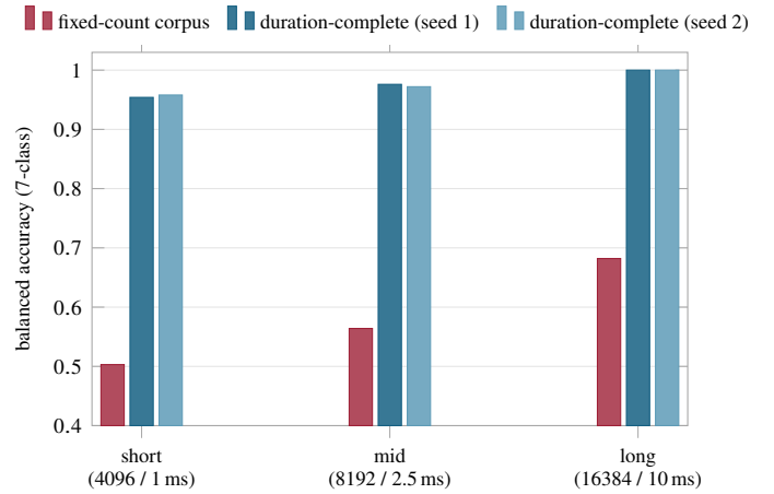
Figure 4: Controlled attribution. The identical 1.0M-parameter encoder, recipe, and budget on the fixed-count control corpus (window tiers in samples) vs. duration-complete data (dwells in milliseconds); tiers are matched by rank, not physical duration, which fixed-count data cannot hold constant. At 10 ms every class reaches recall 1.000 on both seeds.
