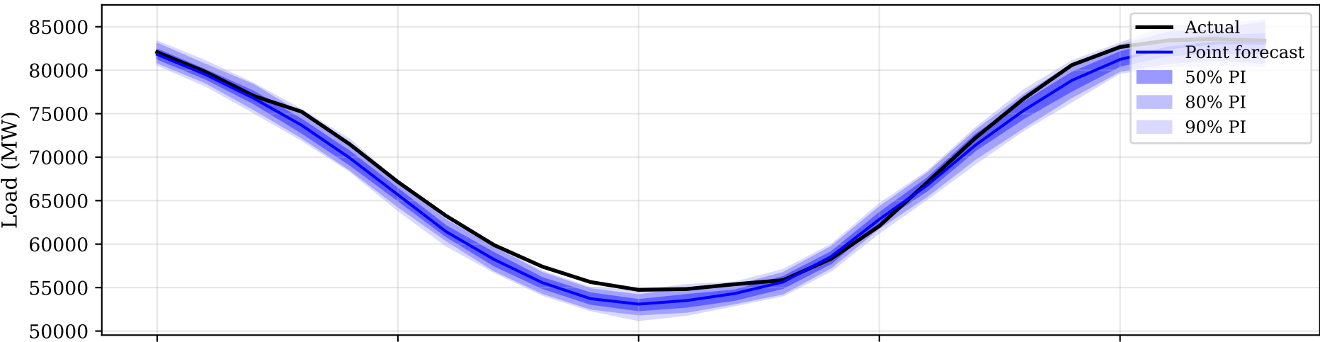
Chronos-2
