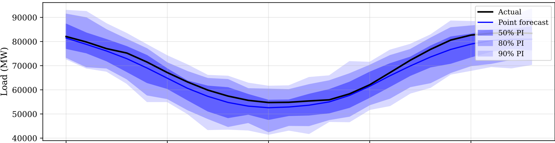
Prophet
