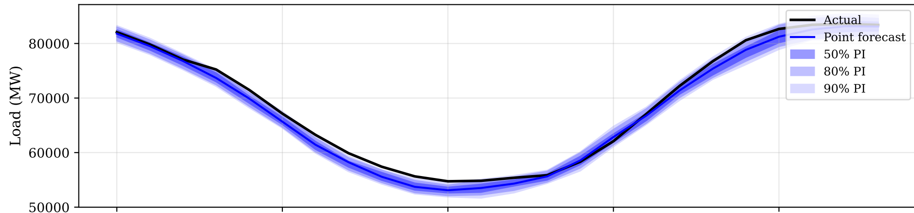
Chronos-2
