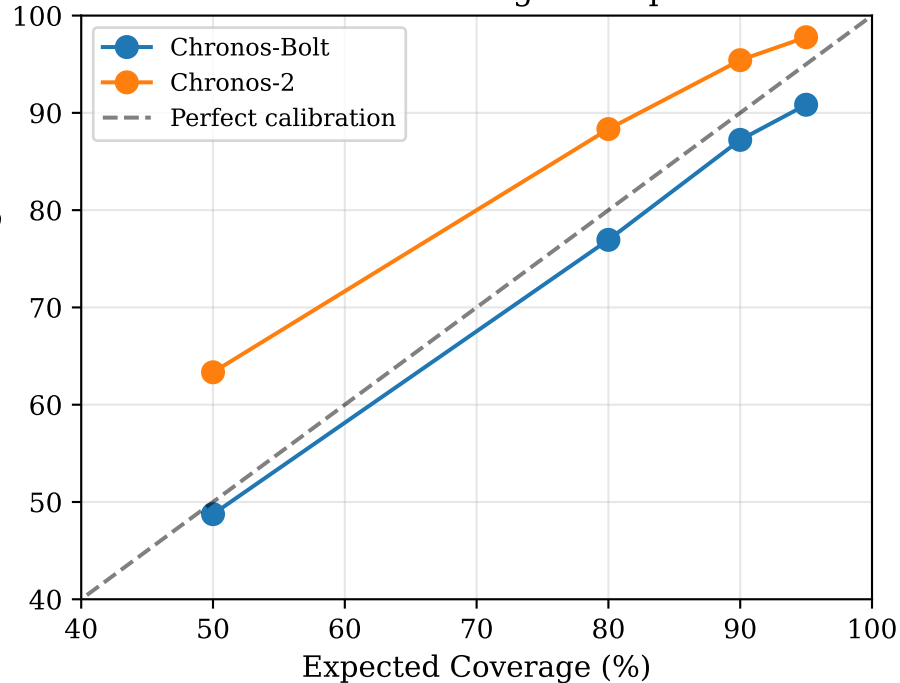
Calibration: Coverage vs Expected
