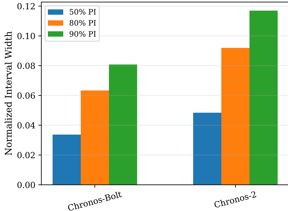
Prediction Interval Width
