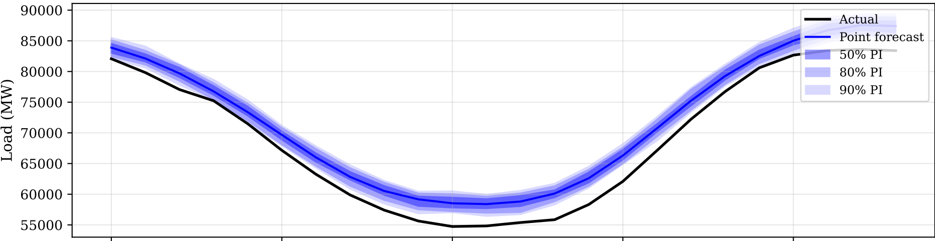
Prophet
