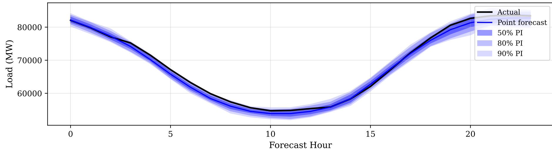
Chronos-2
