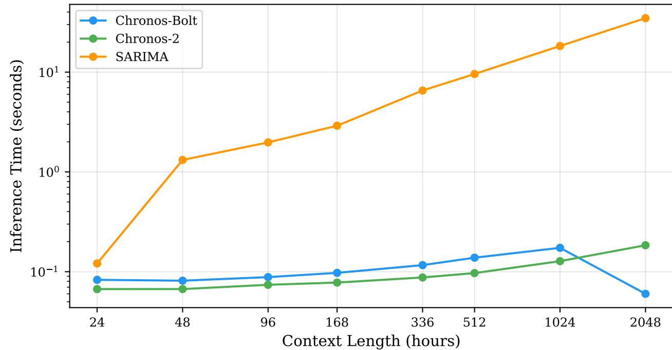
Computational Cost: Inference Time vs Context Length
