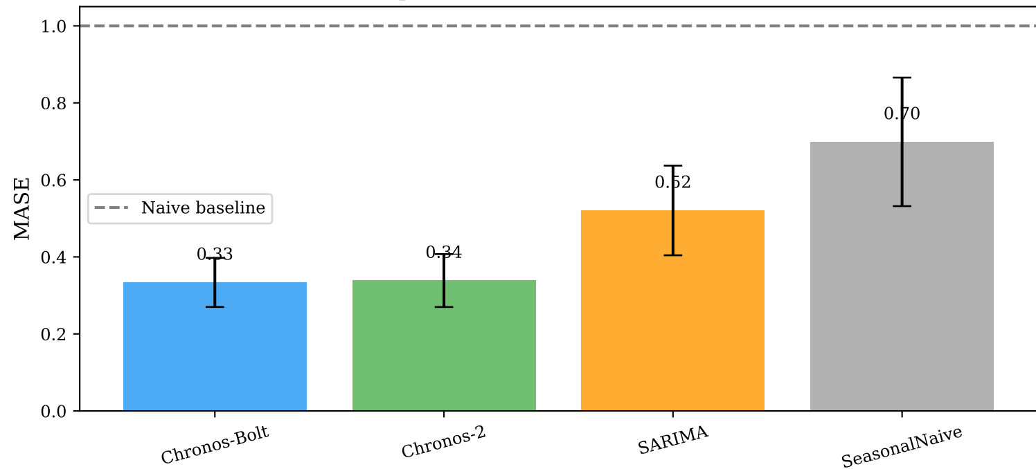
Model Comparison at Context=512h, Horizon=24h
