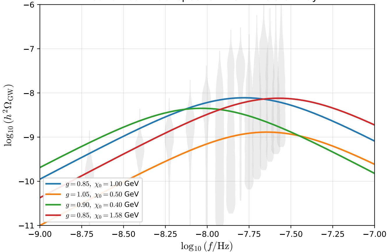
su2cw-dark: dbf spectrum vs NANOGrav 15yr
