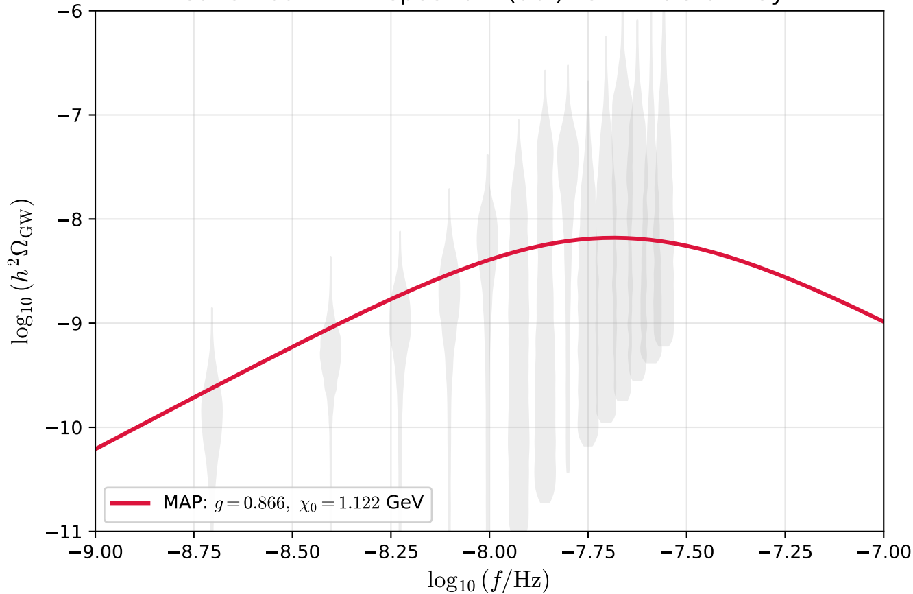
su2cw-dark MAP spectrum (dbf) vs NANOGrav 15yr
