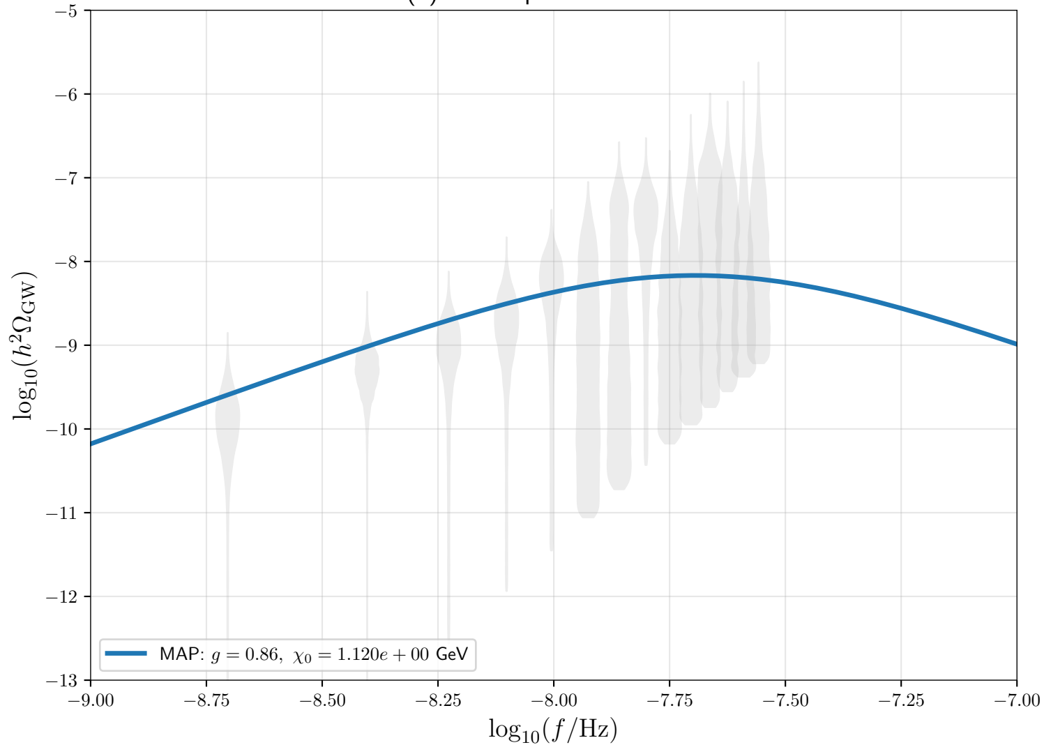
Conformal SU(2) MAP Spectrum vs NANOGrav Violins
