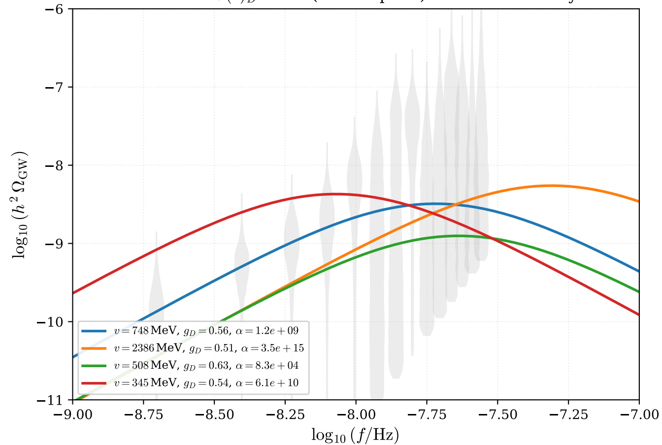
Conformal U(1)_D FOPT (dbf template) vs NANOGrav 15yr
