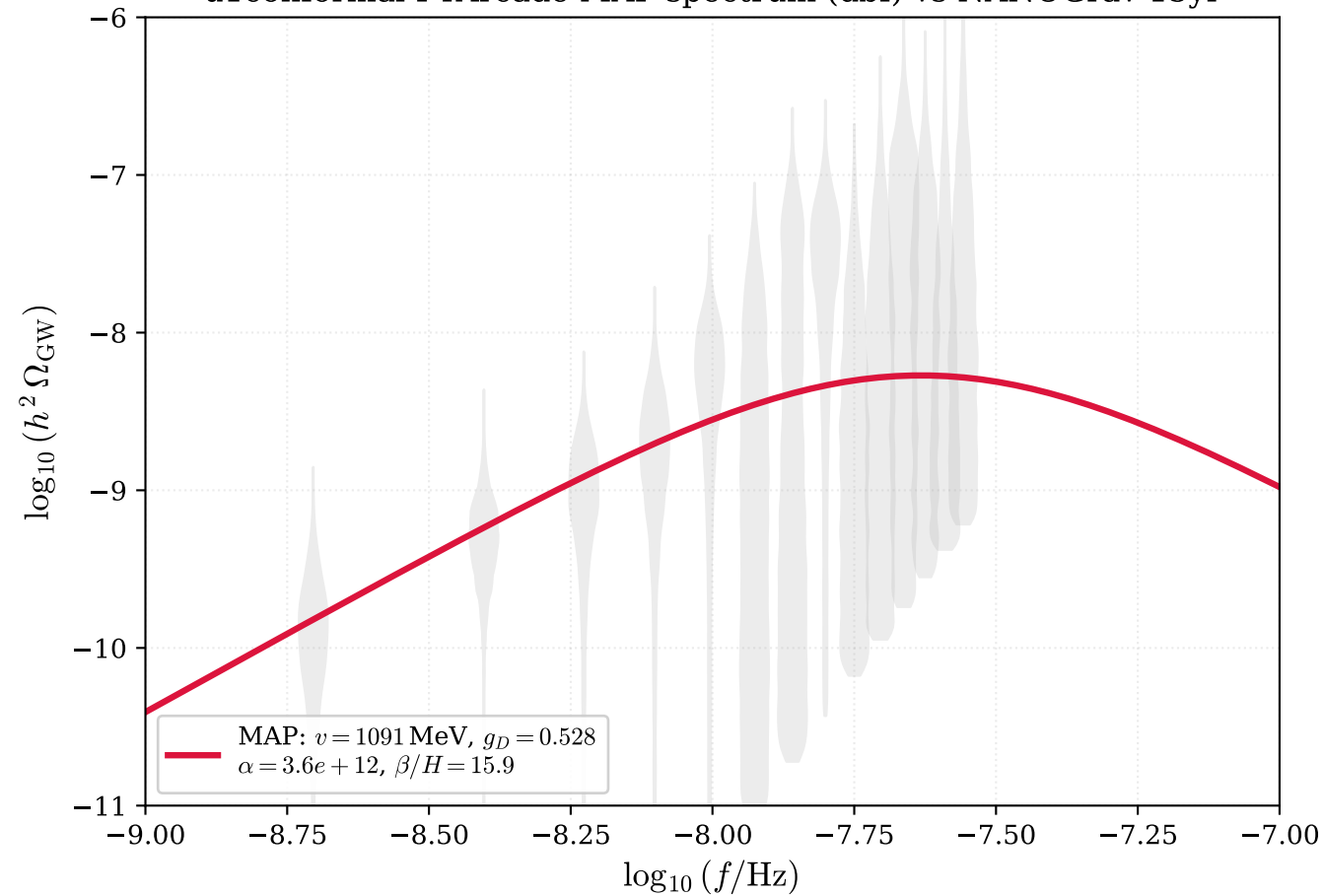
u1conformal PTArcade MAP spectrum (dbf) vs NANOGrav 15yr
