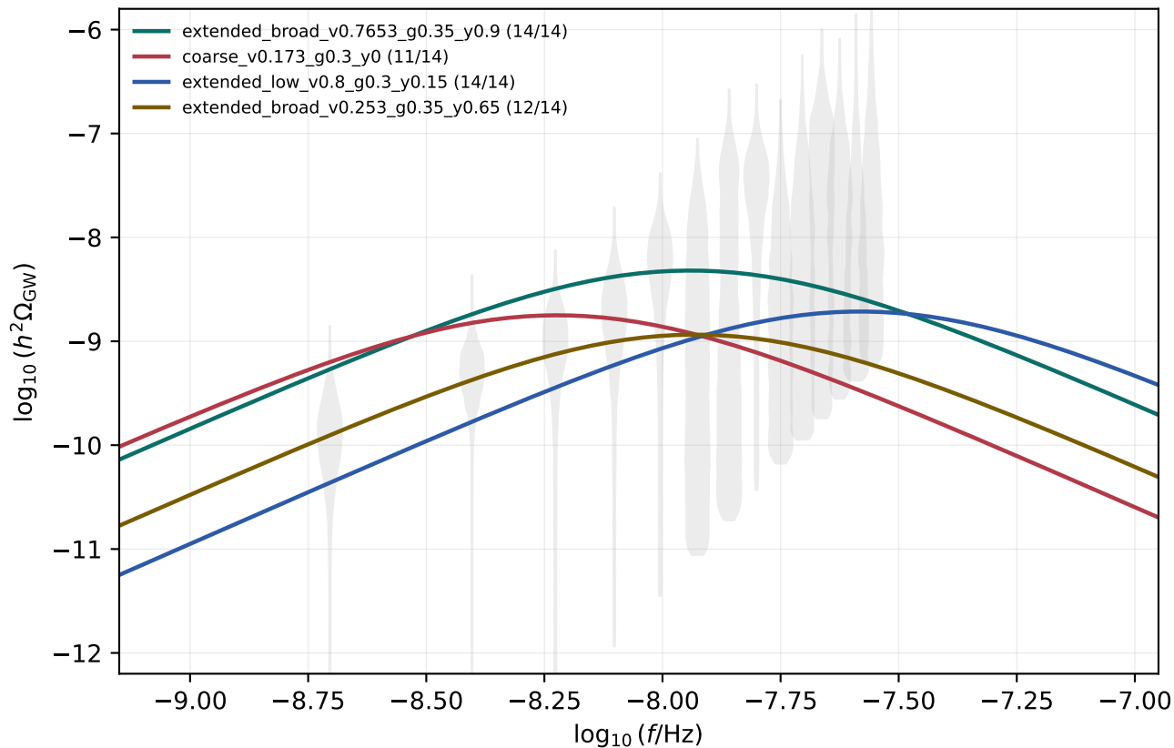
Conformal U(1)_D FOPT benchmark spectra
