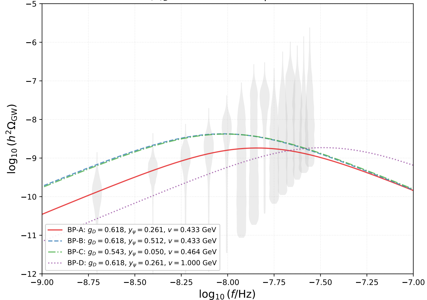
Conformal U(1)_D Dark Sector: GW Spectra vs PTA Violins
