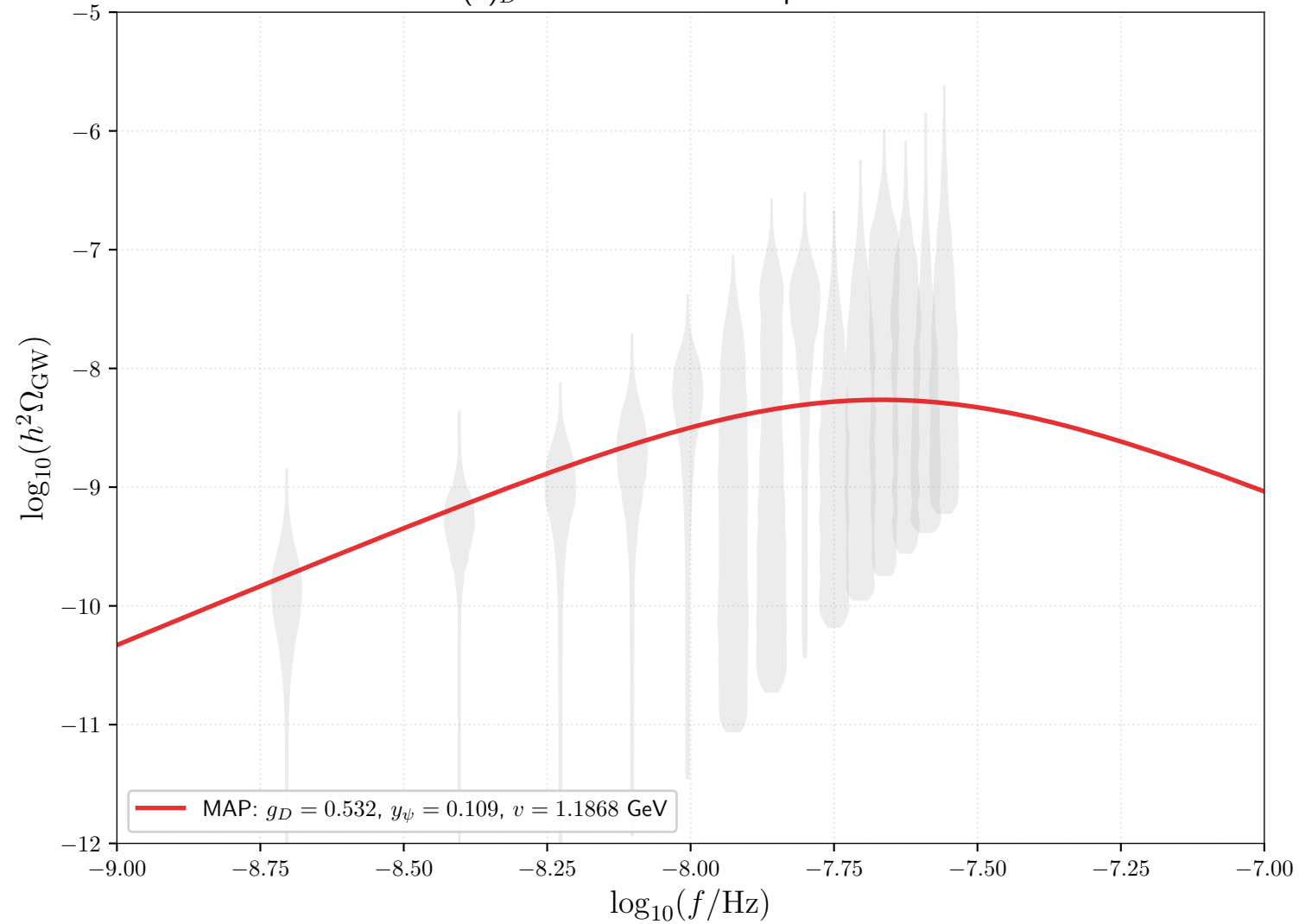
Conformal U(1)_D Dark Sector: MAP Spectrum vs PTA Violins
