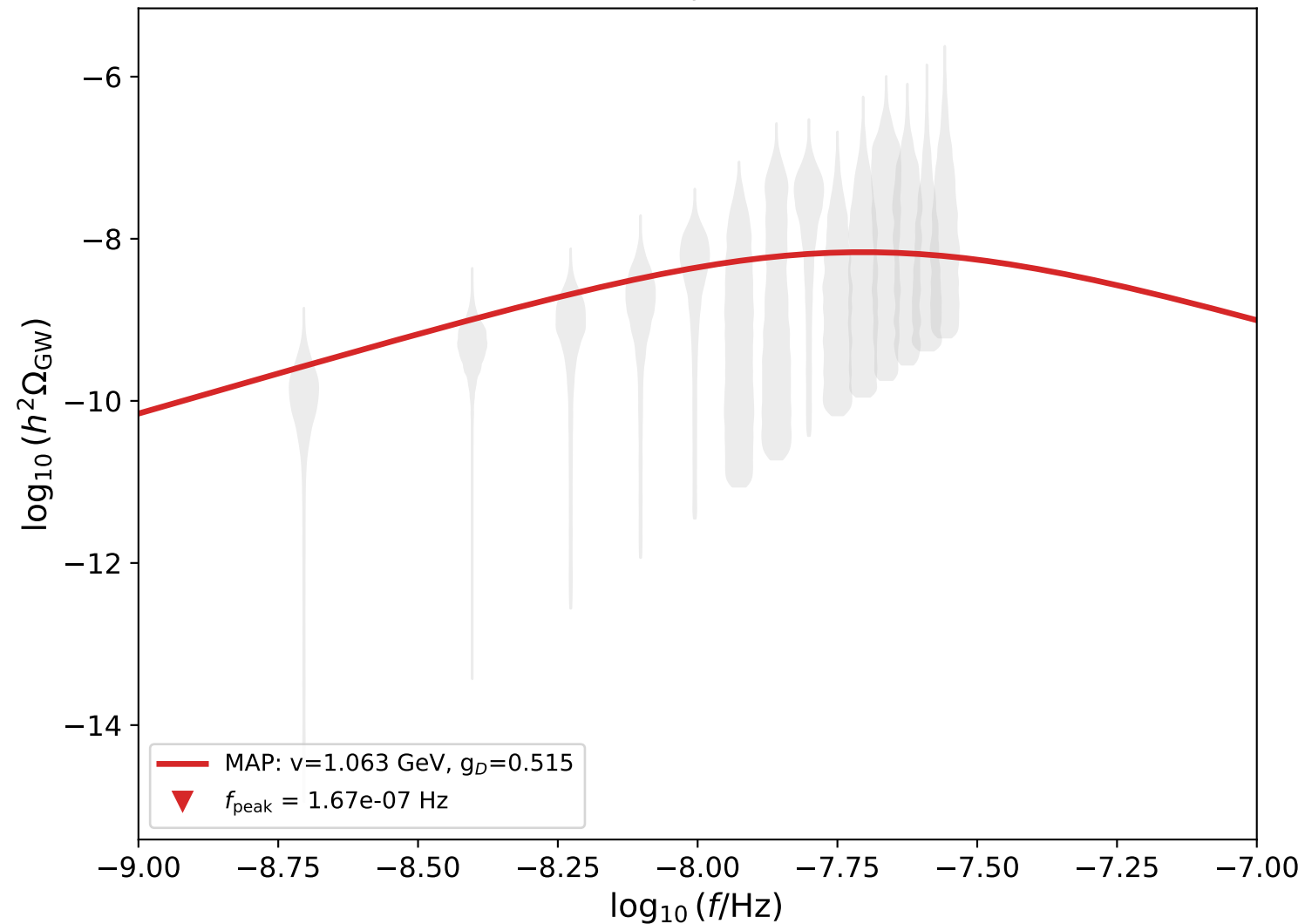
PTArcade MAP Point Spectrum vs PTA Violins
