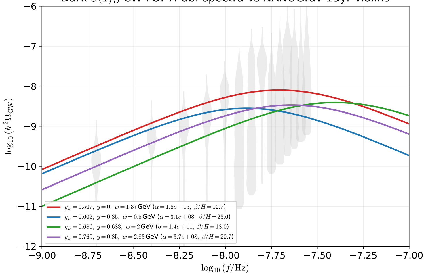
Dark U(1)_D CW FOPT: dbf spectra vs NANOGrav 15yr violins
