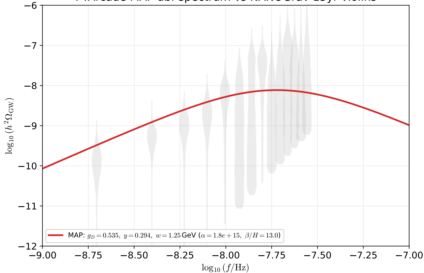
PTArcade MAP dbf spectrum vs NANOGrav 15yr violins
