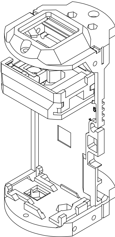
ISOMETRIC VIEW
