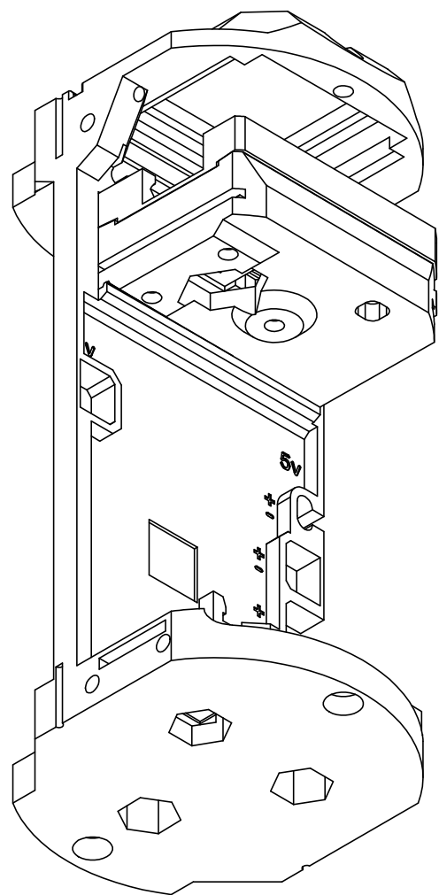
ISOMETRIC VIEW
