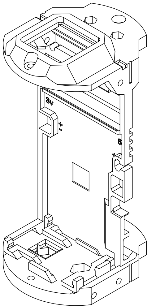
Isometric view
