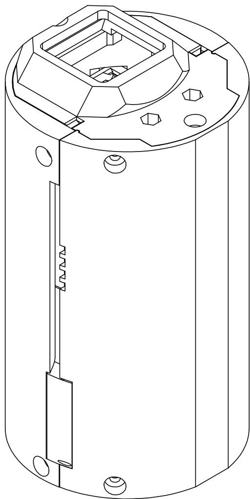
ISOMETRIC VIEW
