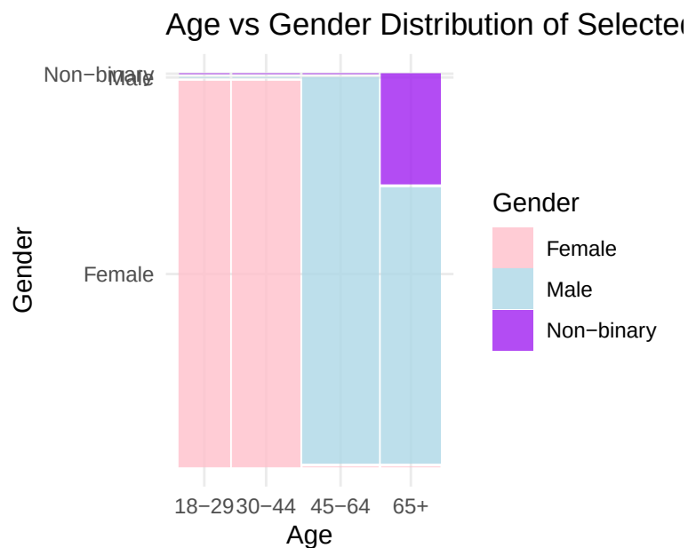
Figure 6: Relationship between age and gender in the selected panel shown as a mosaic plot. Colour indicates gender. Width of the bars correspond to the count within the category. Seven intersections are now not present, and the distribution has shifted significantly from the population and survey sample datasets.
