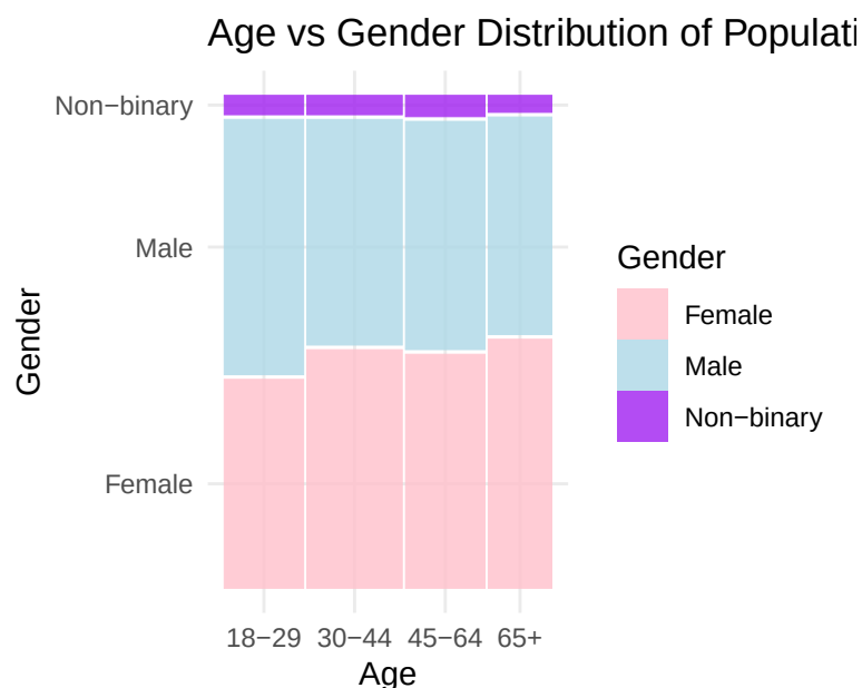
Figure 3: Mosaic plot showing the distribution of age groups across gender in the simulated population dataset
