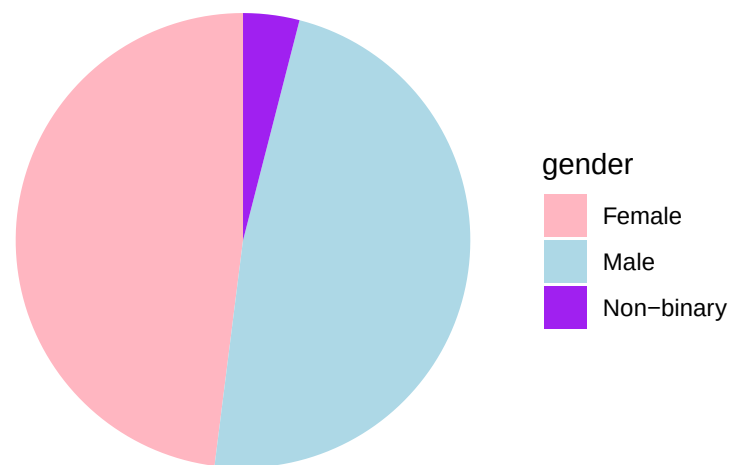
Figure 2: Pie chart showing the distribution of genders in the simulated population dataset
