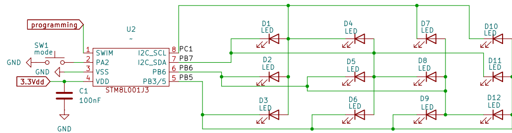
CharliePlexing demo
