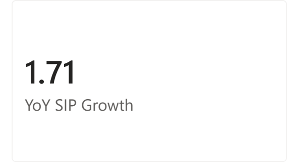
SIP Growth
