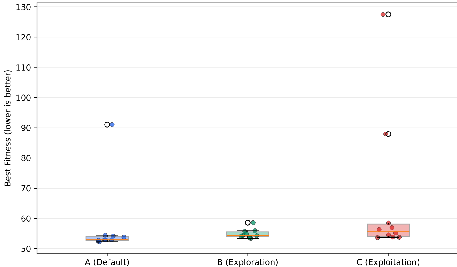
Final Best Fitness by GA Configuration (10 Seeds)
