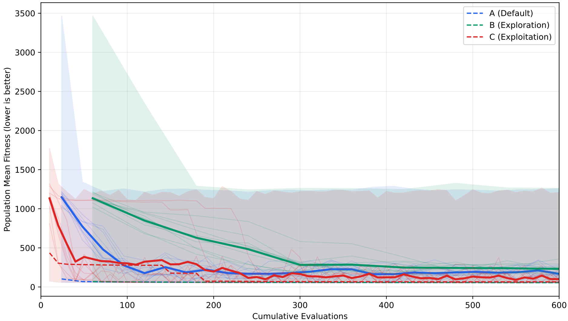
GA Ablation: Population Mean Fitness vs Evaluation Budget
