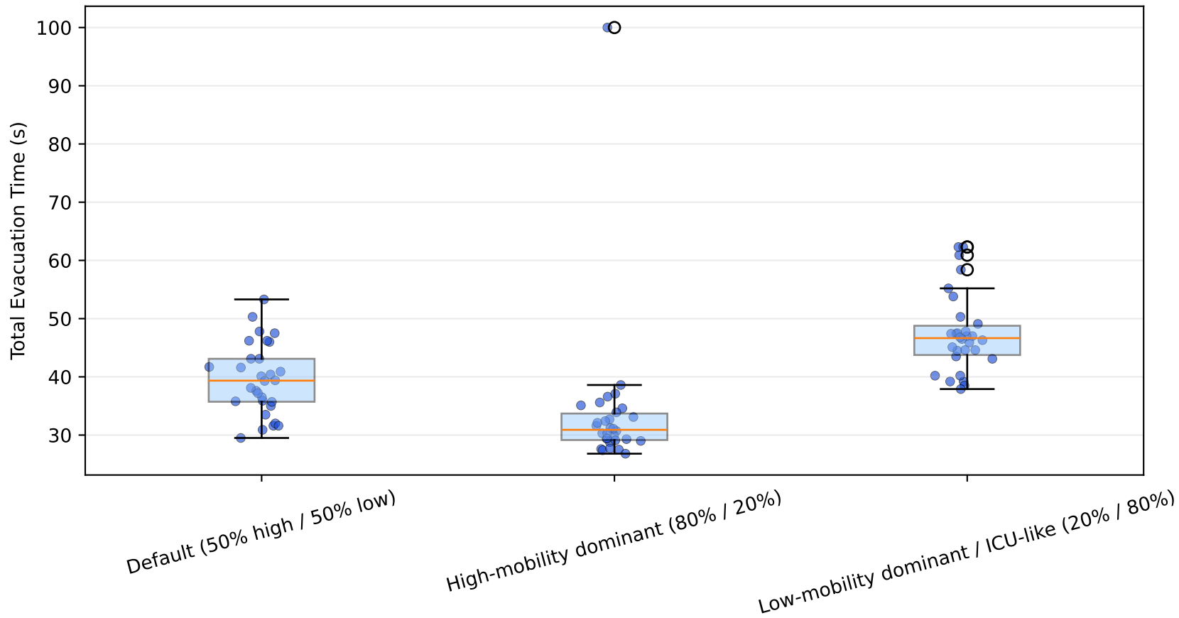
Evacuation Time Across Population Mixtures (Fixed GA Parameters)
